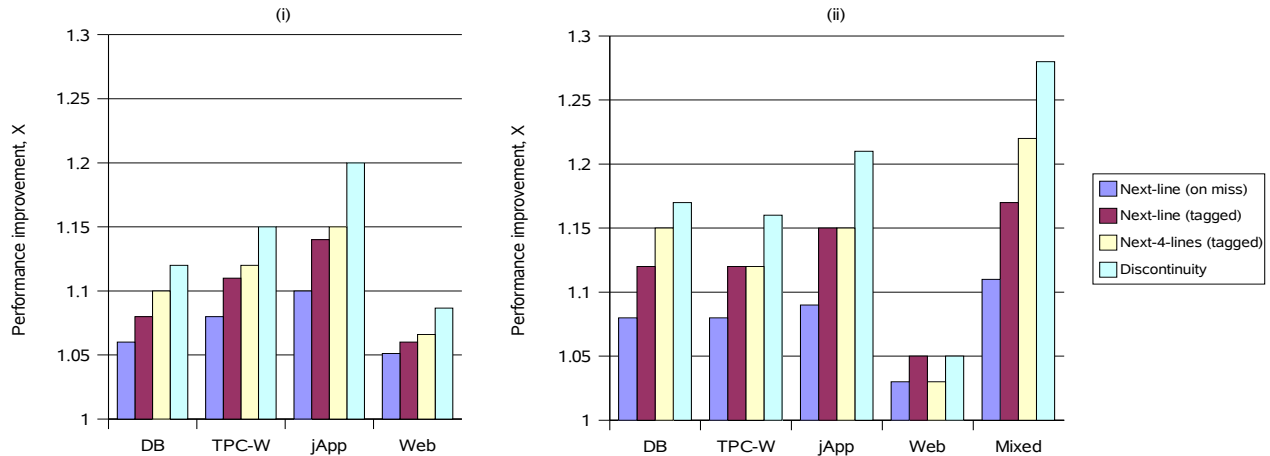
Figure 6. Performance gains achieved by different HW prefetching schemes; (i) single core and (ii) 4-way CMP
